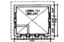
Dimensioned Tower Element SCALE: 1/4" = 1'-0"
