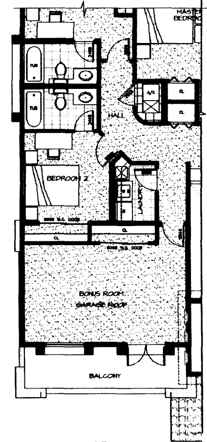
4 2nd. FLOOR PLAN Optional 2 Bathrooms & Bonus Room. SCALE: 1/4" = 1'-0"
