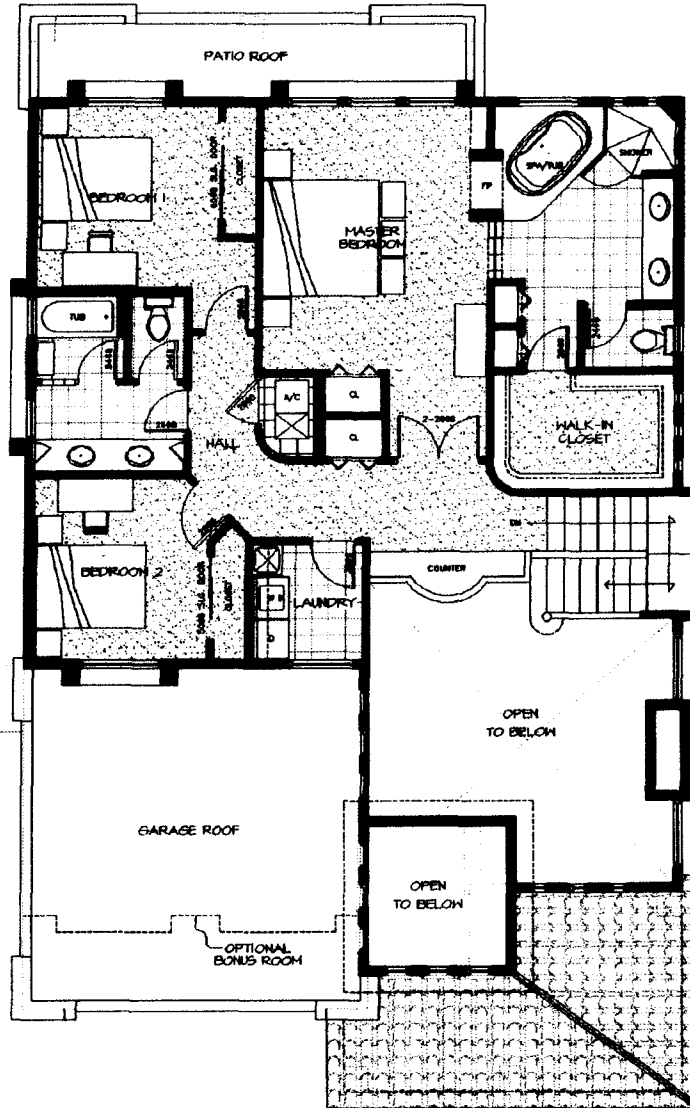
2 2nd. FLOOR PLAN SCALE: 1/4" = 1'-0"
